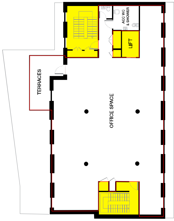
FIFTH FLOOR
