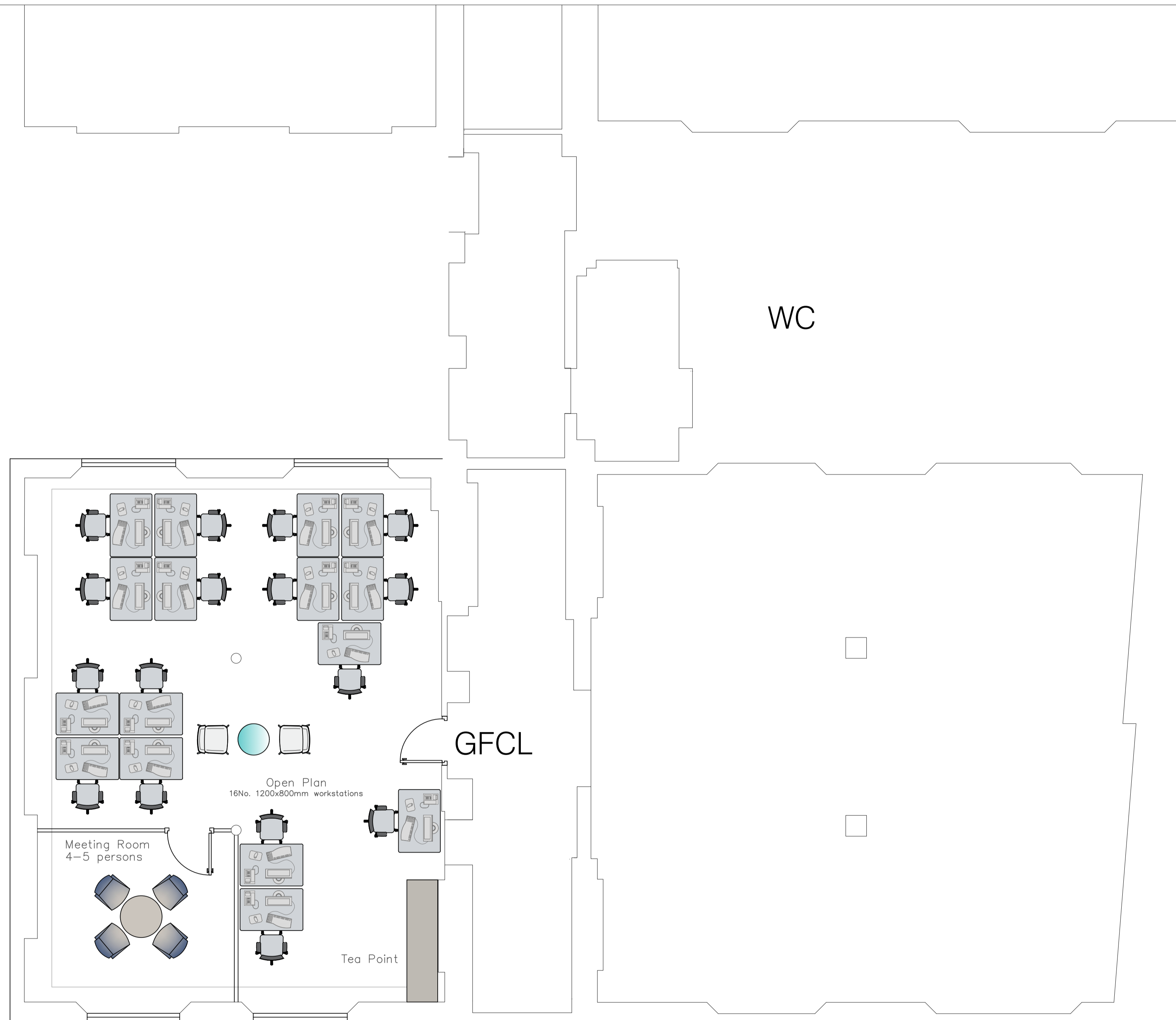
Proposed General Arrangement Plan Ground Floor Desk 1200mm x 800mm
